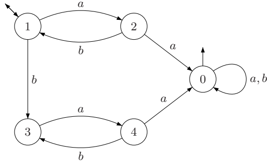
Fig. 2. The minimal automaton of (ab)^* \cup A^*aaA^*
