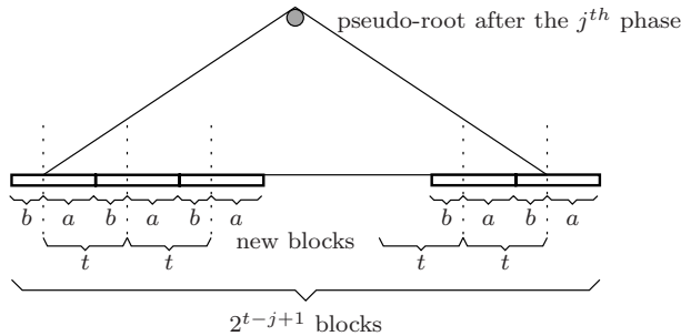
Fig. 5. Relabeling of the blocks after a phase
