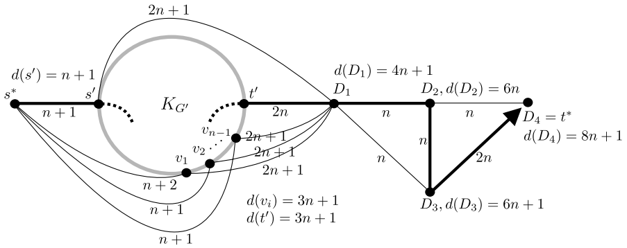
Fig. 4. The graph G^* before the local modification is applied and an optimal Hamiltonian path from s^* to t^*
