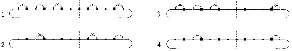
Fig. 1. A sample phase of the ring broadcasting algorithm. The initially active vertices are squares. In the first step, the only surviving message is delivered to the white vertex on the left, which then replies in the next step. At the end of the phase, two white vertices are sending acknowledgement, so at least one acknowledgement is delivered during that phase.
