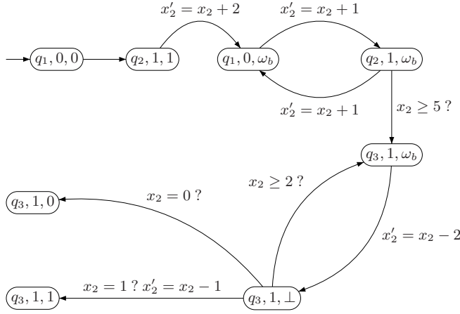
Fig. 3. A 1-reversal-0-bounded counter machine obtained from the counter machine of Fig. 2
