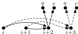
Fig. 3. The template T_{left} , and associated 0/1 values
