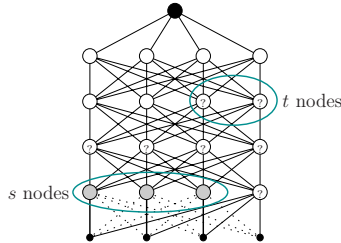
Fig. 2. A partially played T_5^4 and the strategy given in Lemma 1
