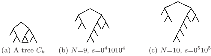
Fig. 2. The class of trees with the longest synchronizing string for a given number of nodes n . s denotes the synchronizing string for each tree. The triangle denotes a code \{1, 01, 001, \dots, 0^i 1, 0^i 0\} , i \geq 0 .
