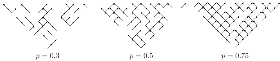
Fig. 2. Oriented percolation with different probability of open bonds
